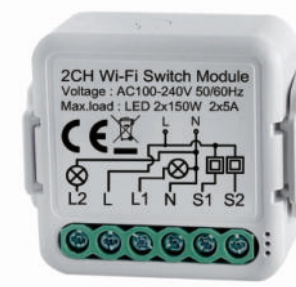
M-2CH 2 Gang Switch
