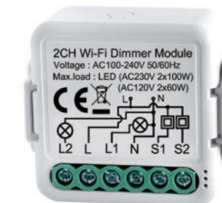
M-2DM 2 Gang Dimmer
