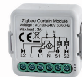
MZ-1CM 1 Gang Curtain
