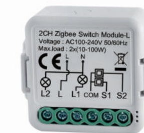
MZ-2CH-L 2 Gang Switch Single Live
