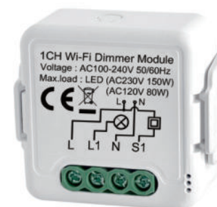
M-1DM 1 Gang Dimmer
