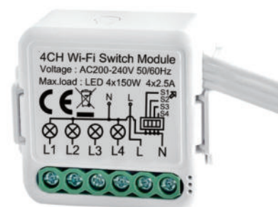
M-4CH 1 Gang Switch
