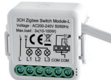
MZ-3CH-L 3 Gang Switch Single Live
