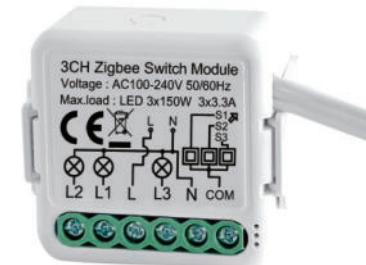
MZ-3CH 3 Gang Switch
